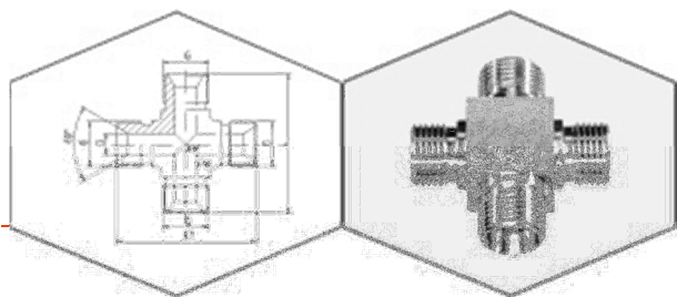
Male - BSP - All sides with 60°-Cone
