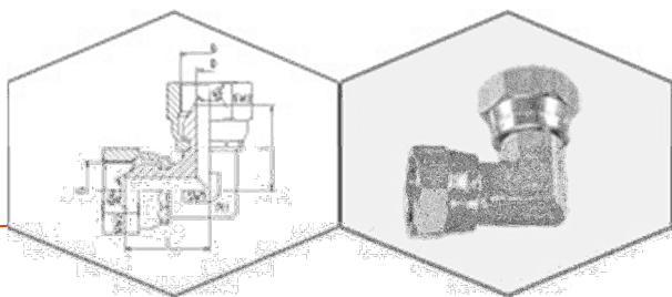
Female - BSP - BSP with Swivel Nut at both sides
