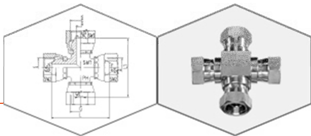
Female - BSP - All sides with Swivel Nut
