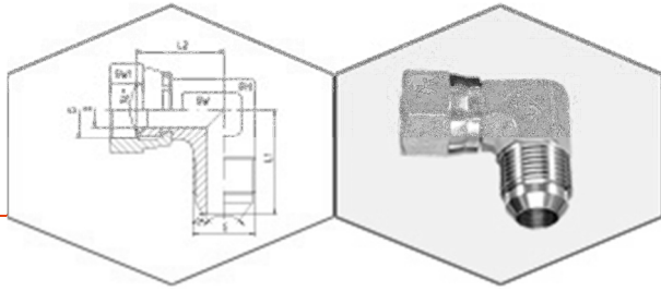
Swivel-Elbow-Adaptors - 90°
