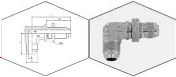
90°-Elbow Bulkhead Connections
