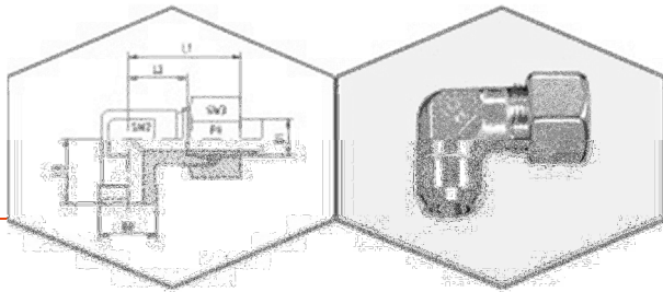
Elbow Welding Couplings
